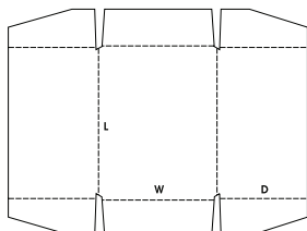
0460 Display Tray or High Wall Tray
