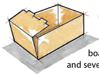
0422 Roll End Tray, Walker Lock Tray, or Tray with Self Locking Ends Formed from a single piece of combined board, the design features an unbroken bottom, and several layers of corrugated in the end panels.
