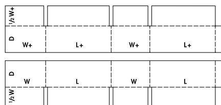
0320 Full Telescope Half Slotted Carton (FTHS)
