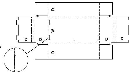
0422 Roll End Tray, Walker Lock Tray, or Tray with Self Locking Ends Formed from a single piece of combined board, the design features an unbroken bottom, and several layers of corrugated in the end panels.
